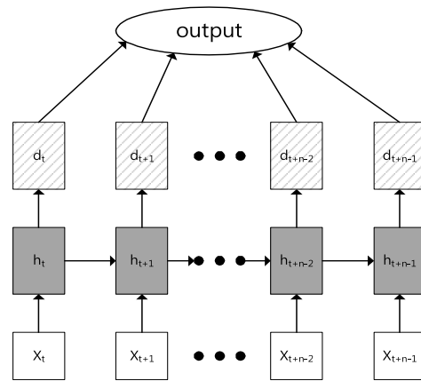
Fig. 1. Basic Structure of RNN
